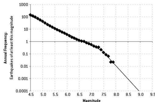
FIGURE 5-7C: TÖHOKU, JAPAN EARTHQUAKE FREQUENCIES CHARACTERISTIC FIT
