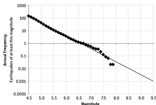
FIGURE 5-7B: TÖHOKU, JAPAN EARTHQUAKE FREQUENCIES GUTENBERG-RICHTER FIT
